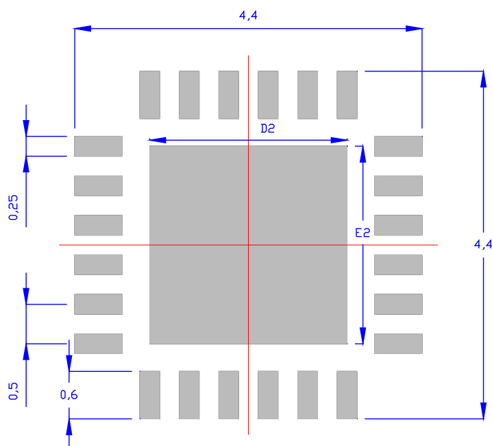
Figure 31. QFN24 4x4x1pitch 0.5 mm PCB pad pattern
