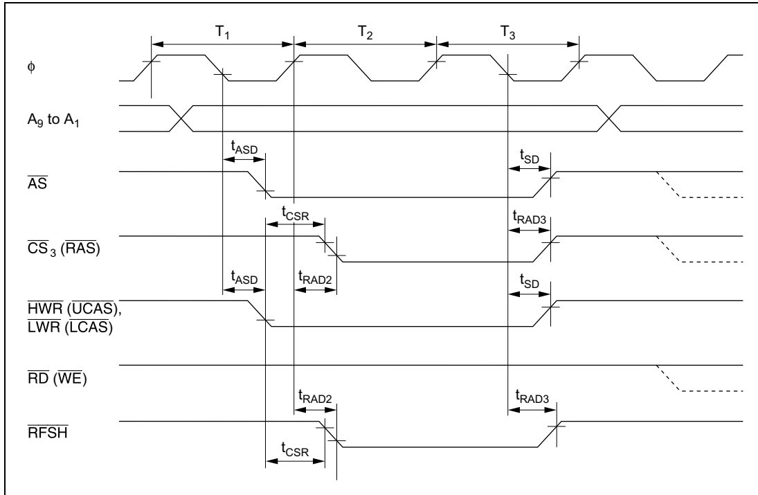
Figure 21.14 DRAM Bus Timing (Refresh Cycle): Three-State Access — 2\overline{CAS} Mode —
