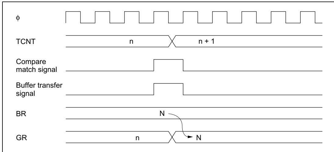
Figure 10.50 Compare Match and Buffer Transfer Timing (Example)
