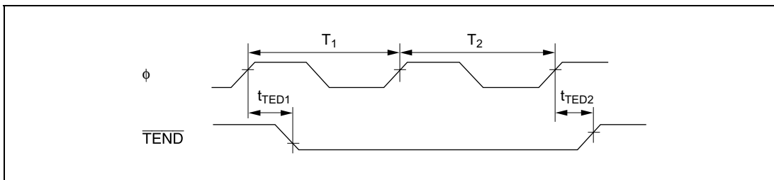
Figure 21.28 DMAC \overline{\text{TEND}} Output Timing for 2 State Access
