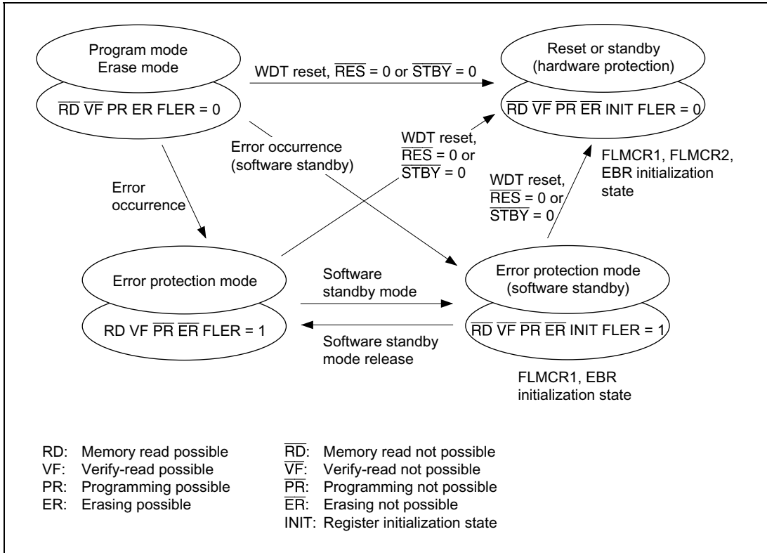
Figure 18.15 Flash Memory State Transitions (When High Level is Applied to FWE Pin in Mode 5, 6, and 7 (On-Chip ROM Enabled))
