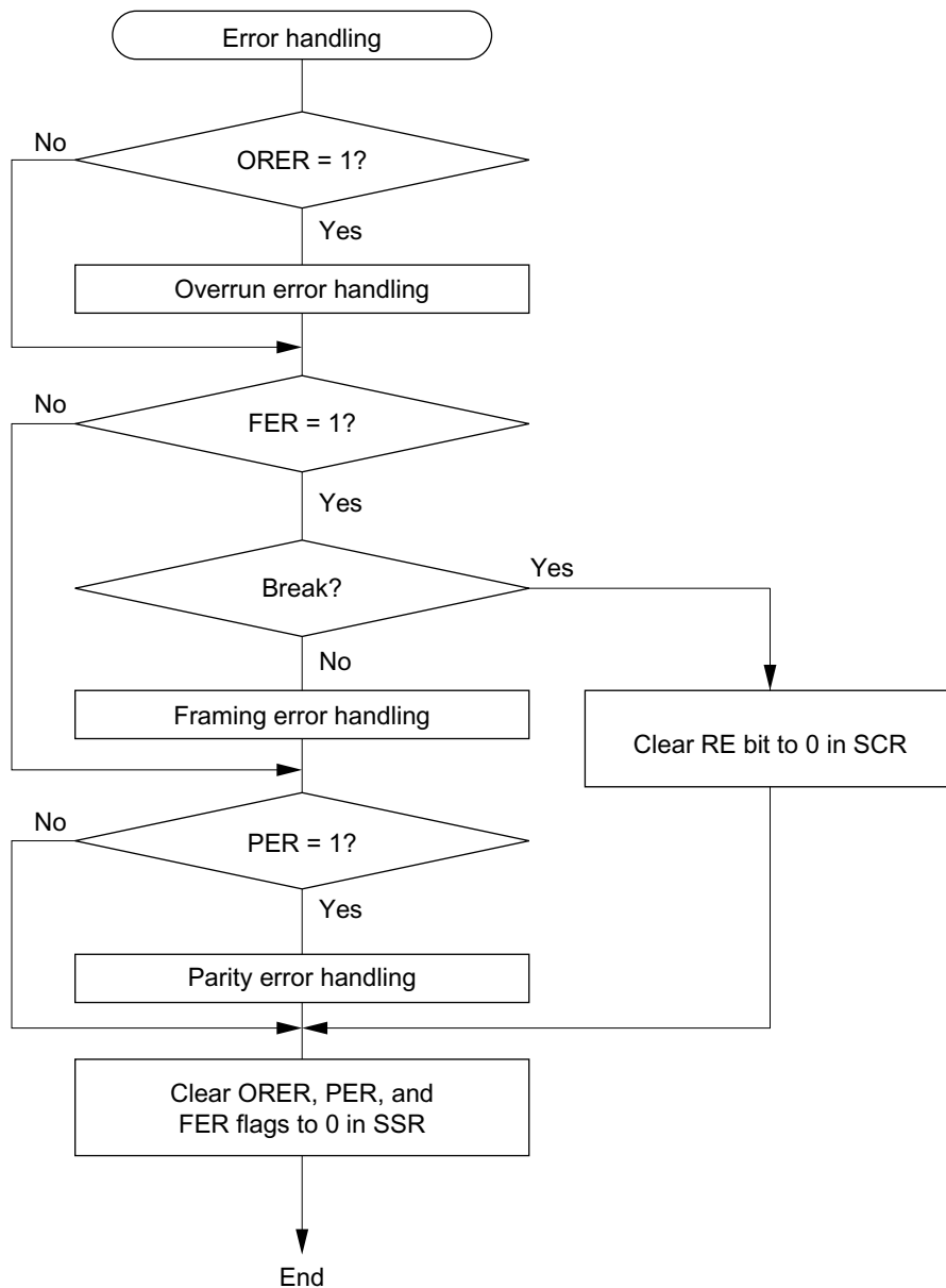
Figure 13.7 Sample Flowchart for Receiving Serial Data (2)
