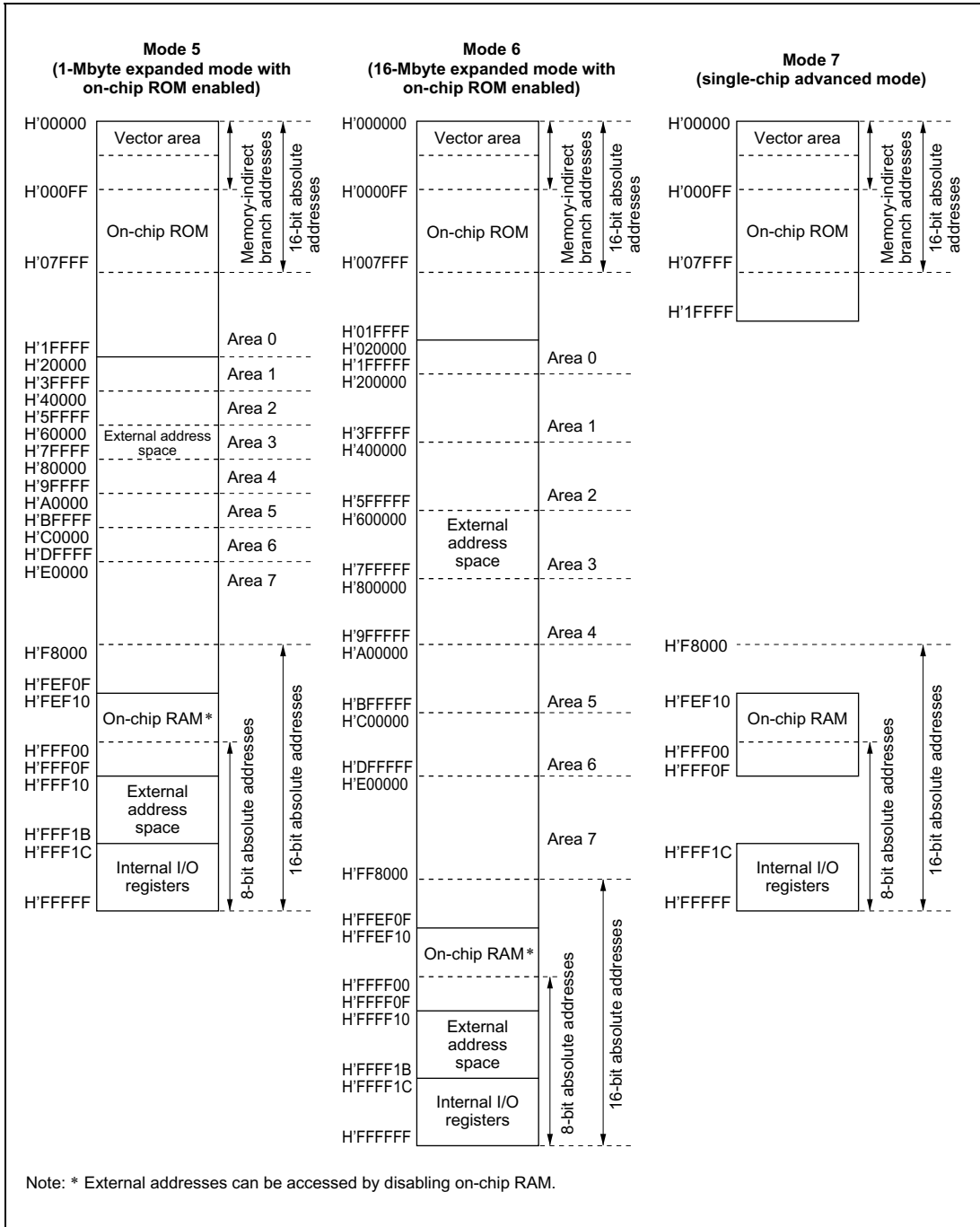
Figure 3.1 H8/3048B Series Memory Map in Each Operating Mode (cont)
