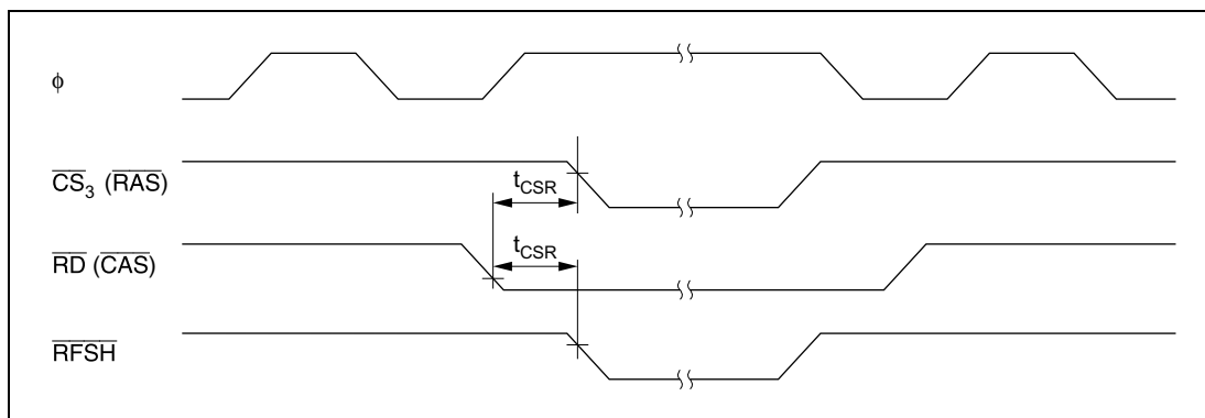
Figure 21.12 DRAM Bus Timing (Self-Refresh Mode) — 2\overline{WE} Mode —
