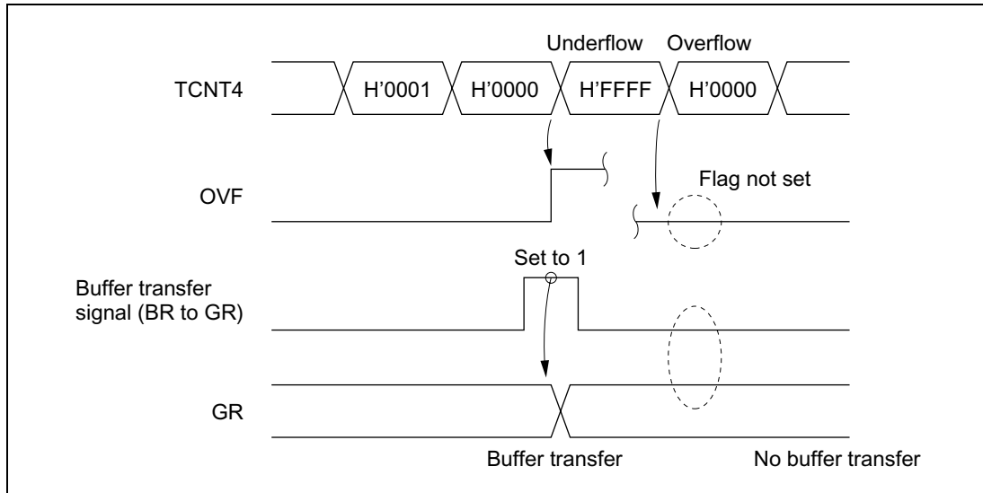
Figure 10.38 Undershoot Timing
