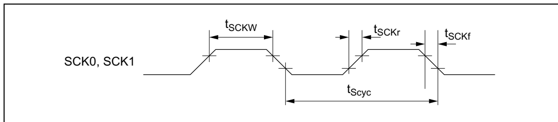
Figure 21.26 SCK Input Clock Timing
