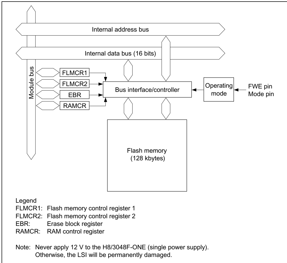
Figure 18.1 Block Diagram of Flash Memory
