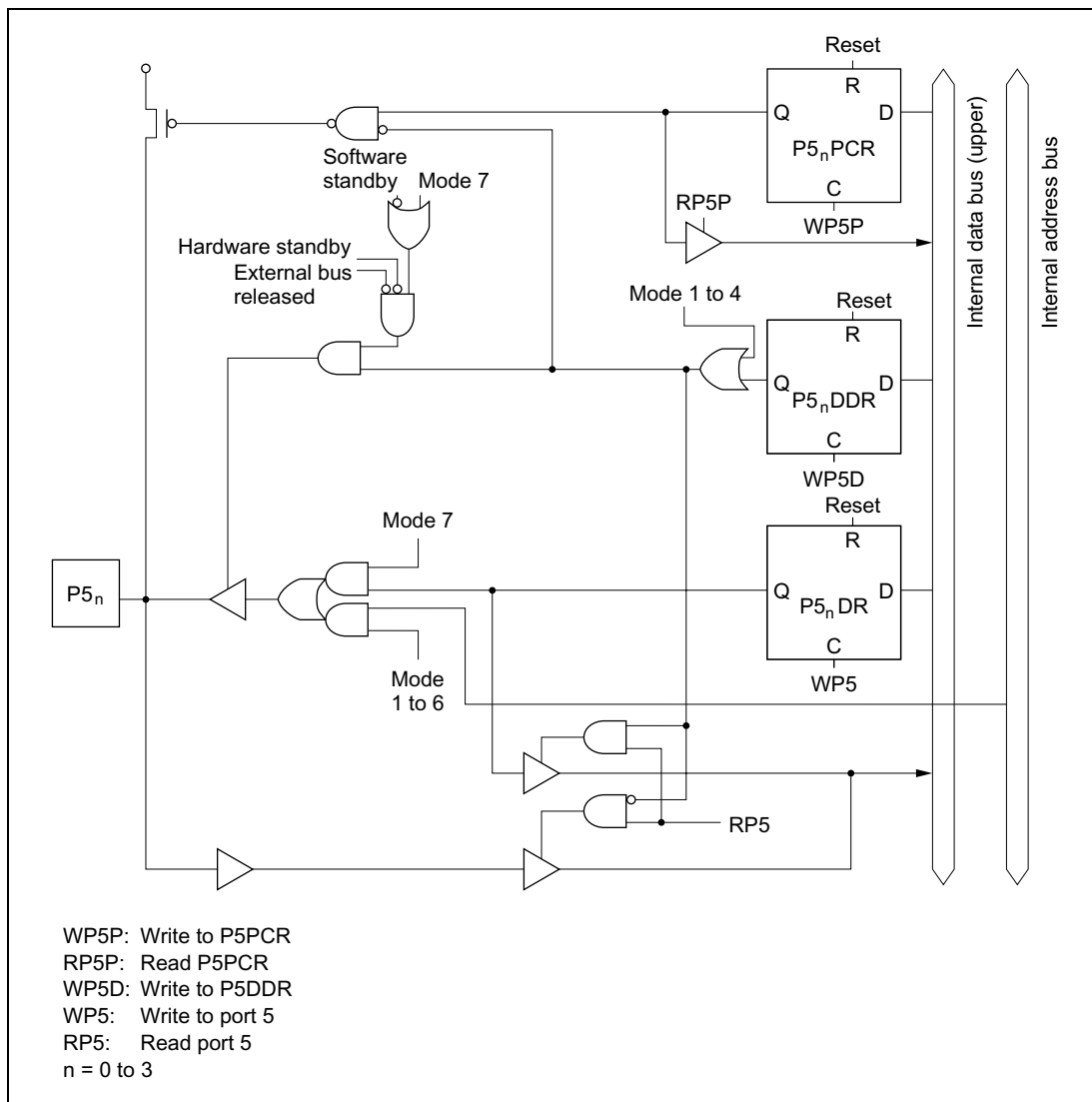
Figure C.5 Port 5 Block Diagram (Pins P5_0 to P5_3 )
