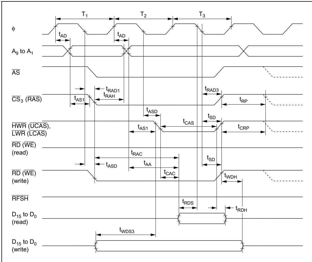
Figure 21.13 DRAM Bus Timing (Read/Write): Three-State Access — 2\overline{CAS} Mode —
