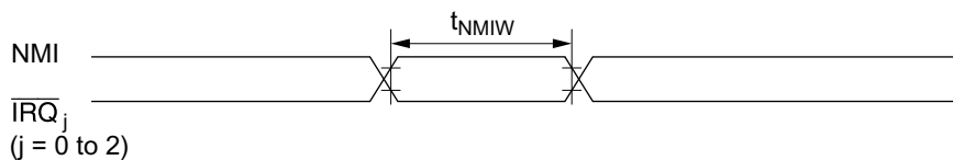
Figure 21.20 Interrupt Input Timing
