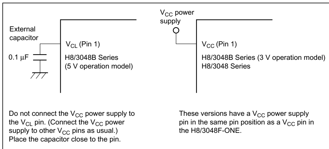
Figure 1.4 Method of Connecting H8/3048B Series V_{CL} Capacitor
