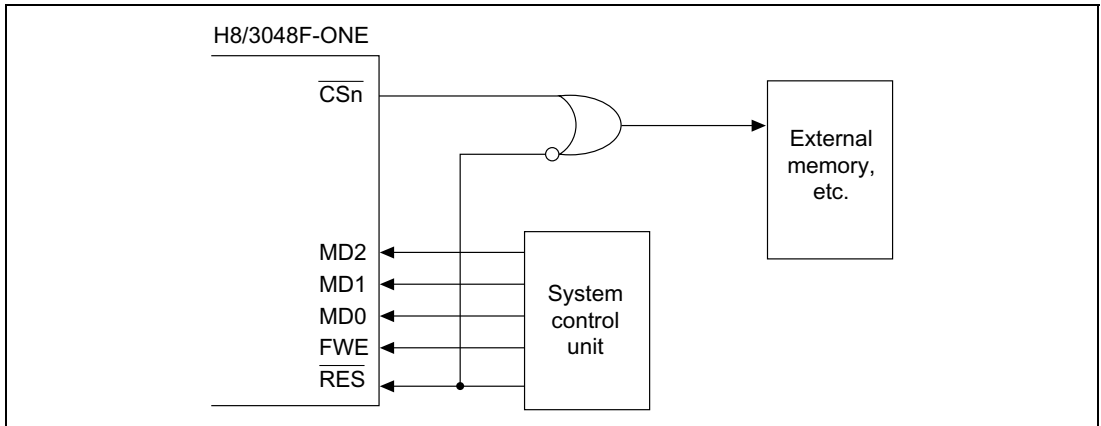
Figure 18.10 Recommended System Block Diagram
