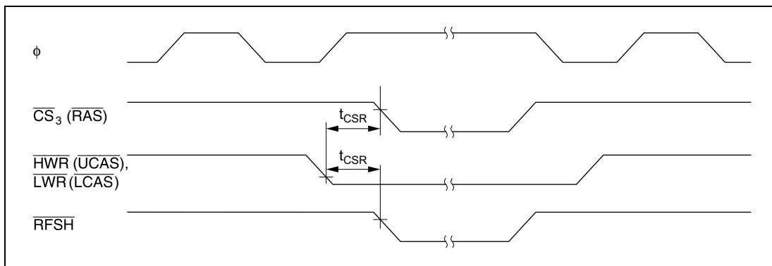
Figure 21.15 DRAM Bus Timing (Self-Refresh Mode) — 2\overline{CAS} Mode —
