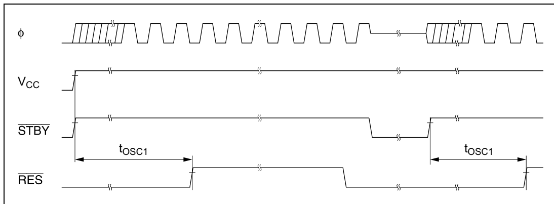
Figure 21.22 Oscillator Settling Timing
