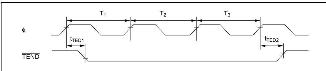
Figure 21.29 DMAC \overline{\text{TEND}} Output Timing for 3 State Access
