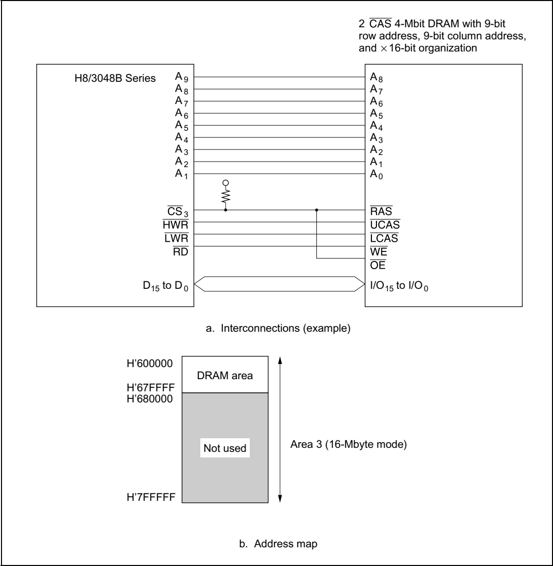
Figure 7.11 Interconnections and Address Map for \overline{2CAS} 4-Mbit DRAM (Example)
