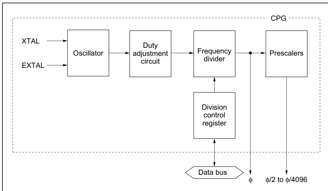
Figure 19.1 Block Diagram of Clock Pulse Generator
