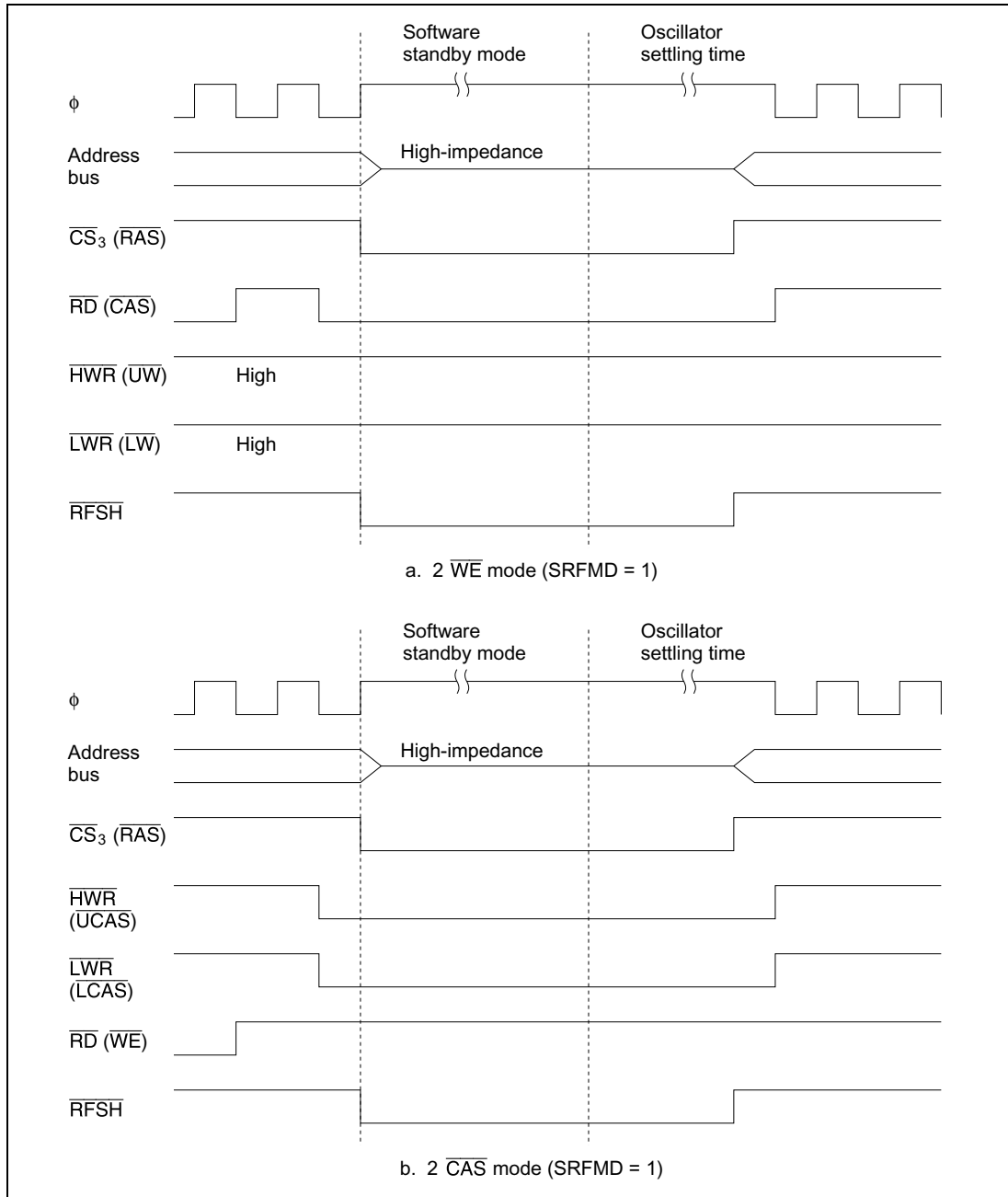
Figure 7.6 Signal Output Timing in Self-Refresh Mode (PSRAME = 0, DRAE = 1)
