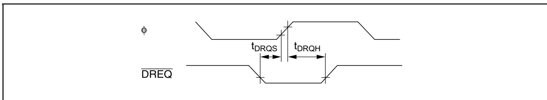
Figure 21.30 DMAC \overline{\text{DREQ}} Input Timing
