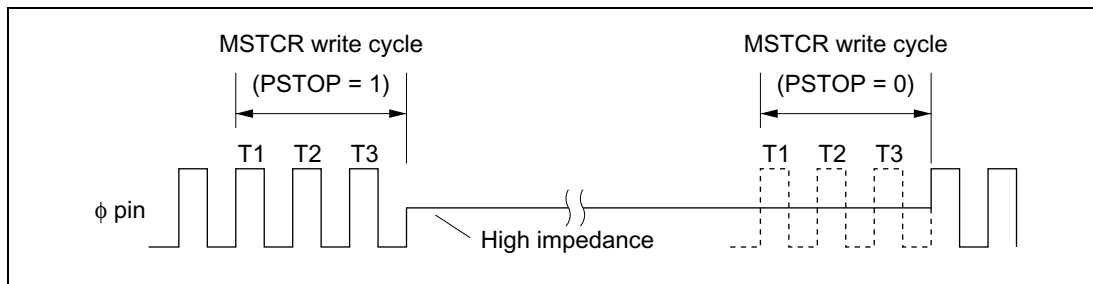
Figure 20.3 Starting and Stopping of System Clock Output
