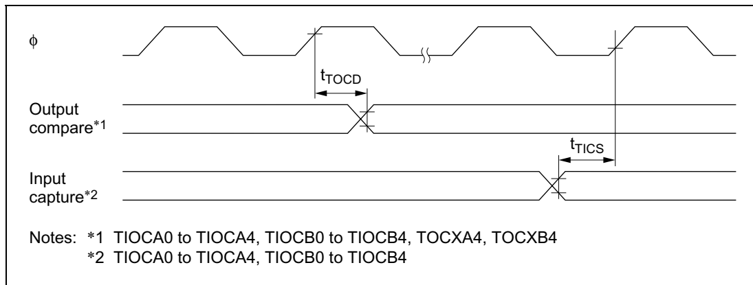
Figure 21.24 ITU Input/Output Timing
