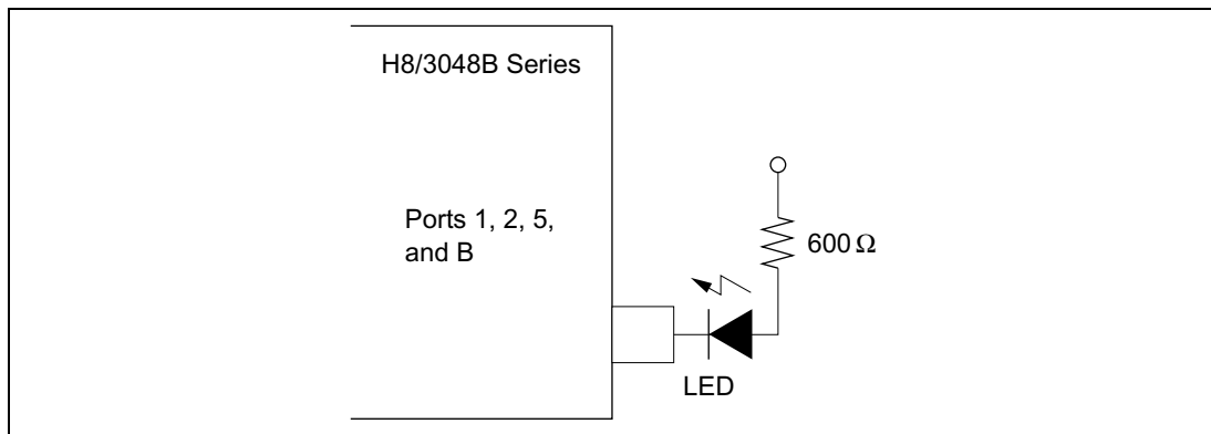
Figure 21.5 LED Drive Circuit (Example)
