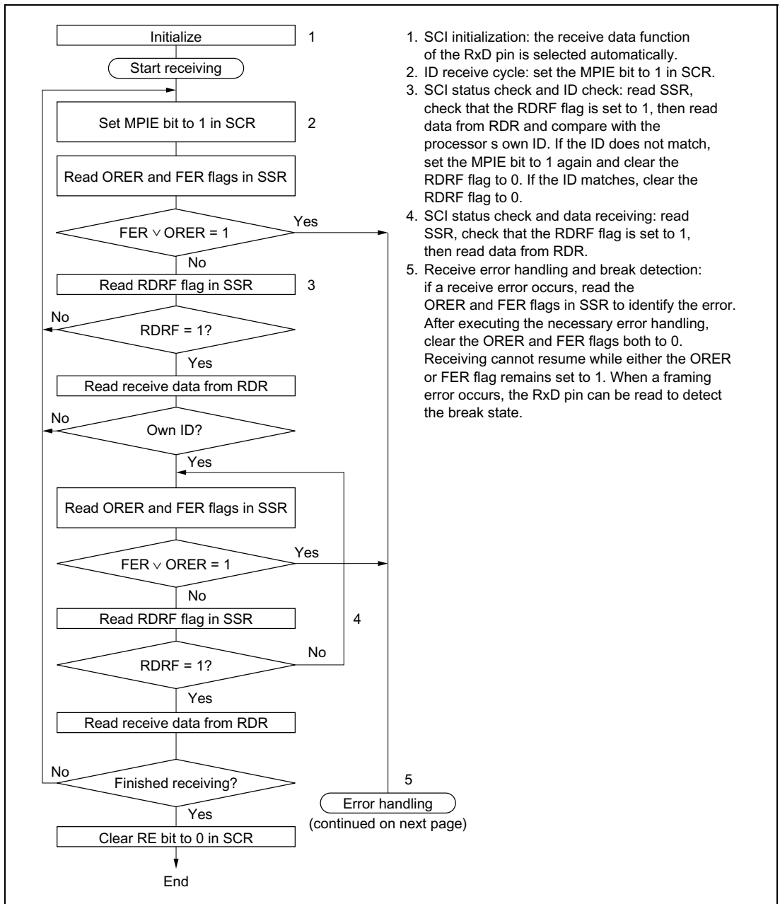
Figure 13.12 Sample Flowchart for Receiving Multiprocessor Serial Data (1)
