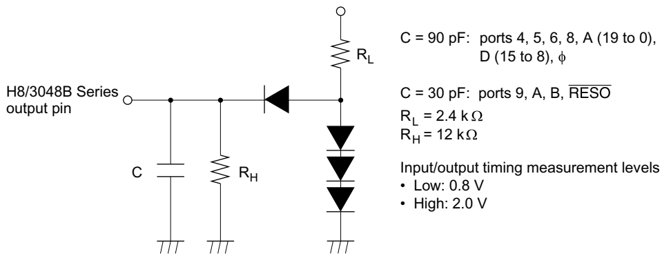
Figure 21.6 Output Load Circuit
