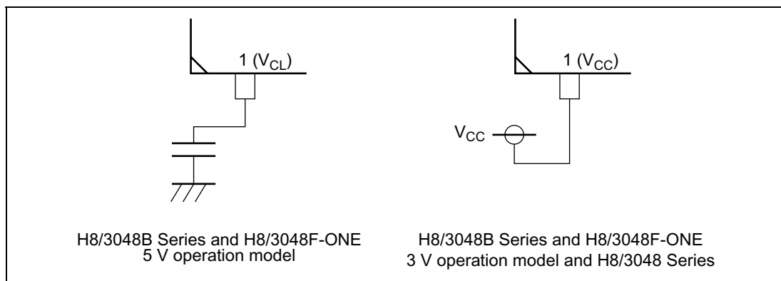
Figure 1.2 Connection of Pin 1
