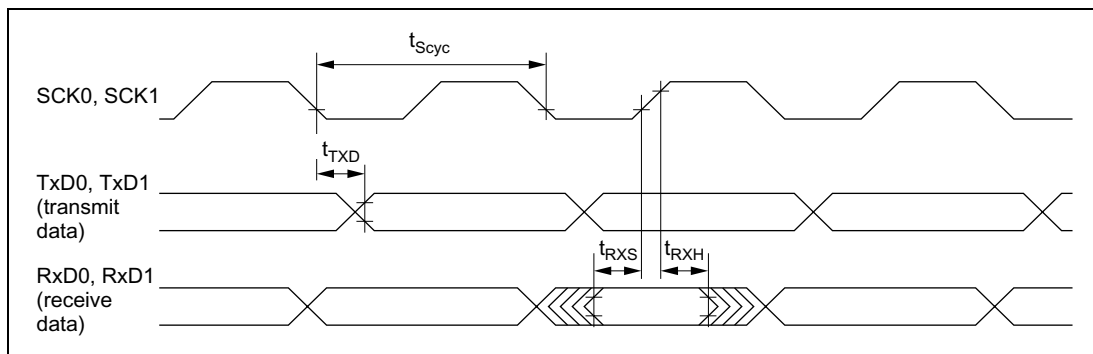
Figure 21.27 SCI Input/Output Timing in Synchronous Mode
