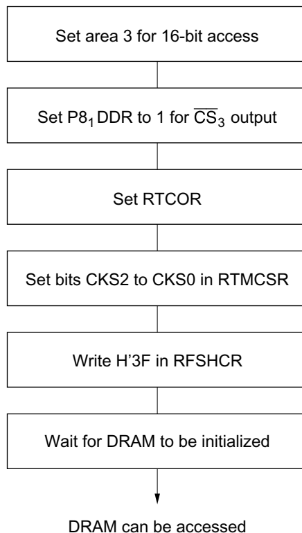
Figure 7.14 Setup Procedure for Multiple 2\overline{CAS} 4-Mbit DRAM Chips with 9-Bit Row Address and 9-Bit Column Address (16-Mbyte Mode)
