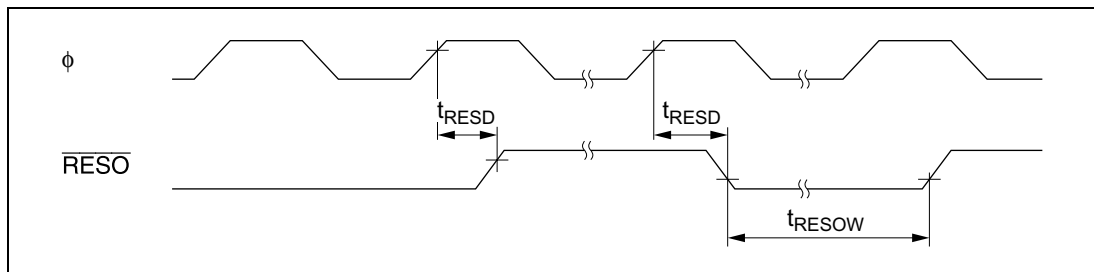
Figure 21.19 Reset Output Timing*
