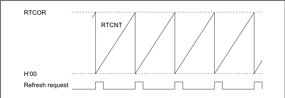
Figure 7.2 Refresh Request Interval (RCYCE = 1)
