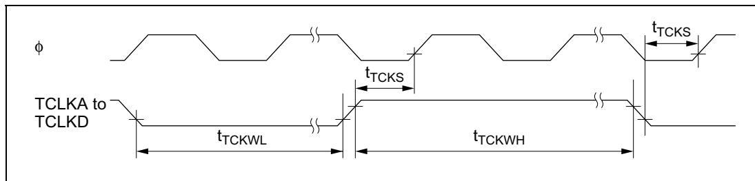
Figure 21.25 ITU External Clock Input Timing
