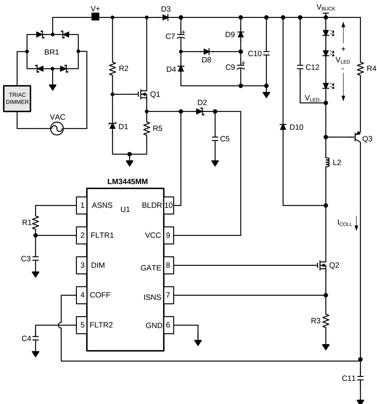
Figure 11. LM3445 Schematic
