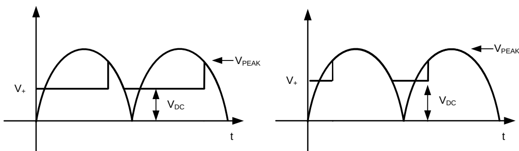
Figure 29. V_{\text{BUCK}} Waveforms With Various Firing Angles
