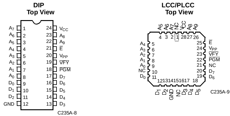
Figure 1. Programming Pinouts.
