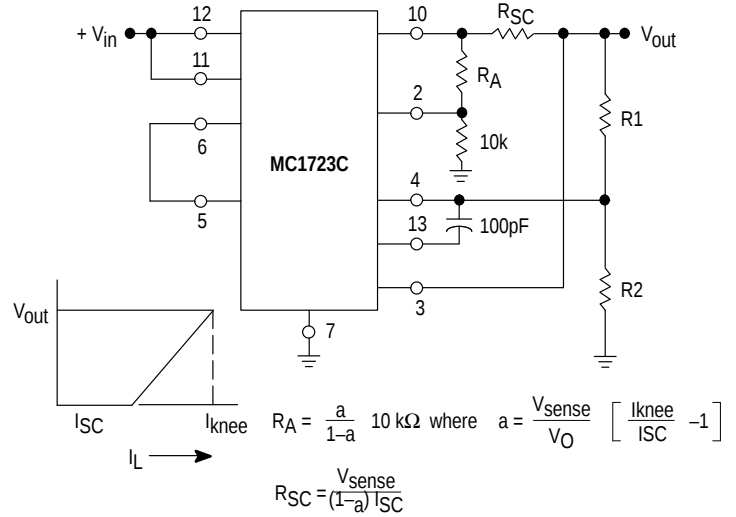
Figure 17. Foldback Connection
