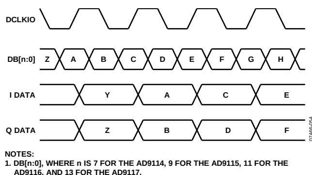
Figure 92. Timing Diagram with IFIRST = 1, IRISING = 1
