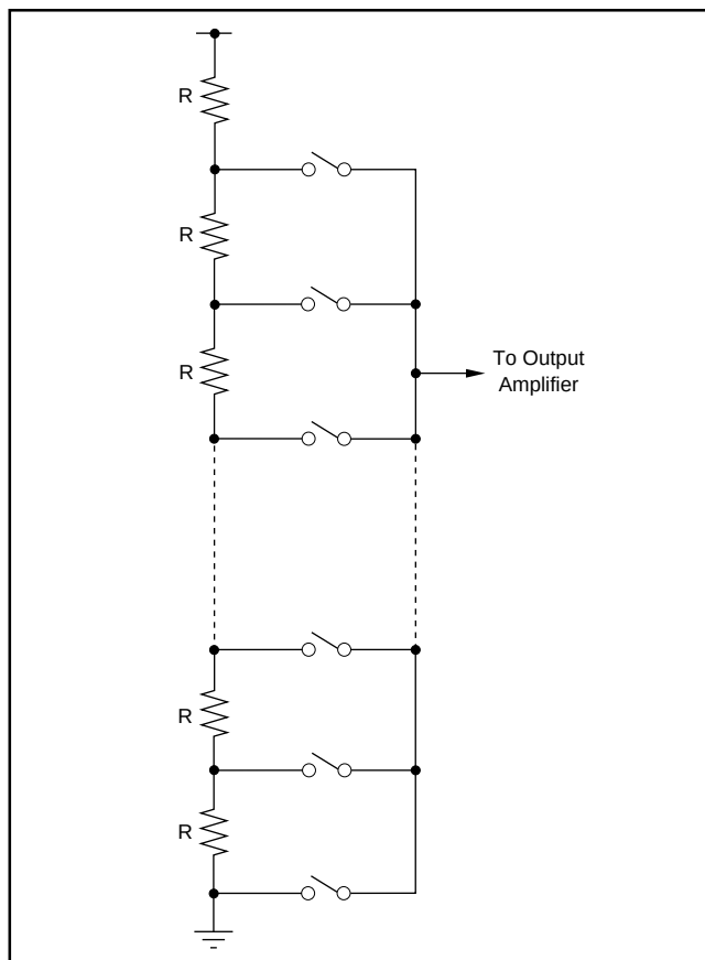
FIGURE 2. Resistor String.
