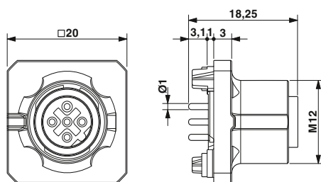
Technical drawing of the M12 connector showing front and side views with dimensions: Front View (Left): Shows a square face with a width of \square 20 . The center features a circular contact area with four small circular pins arranged in a cross pattern. Side View (Right): Shows the profile of the connector with the following dimensions: Overall height: 18,2 Distance from top edge to the first contact pin: 3,1 Distance between the first and second contact pins: 1,1 Distance from the second contact pin to the mounting flange: 3 Mounting flange diameter: \varnothing 1 Thread specification: M12
