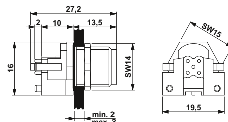
M12 flush-type plug, straight,
