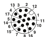
Plug, 17-pos.
