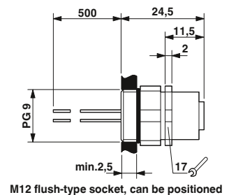
M12 flush-type socket, can be positioned
