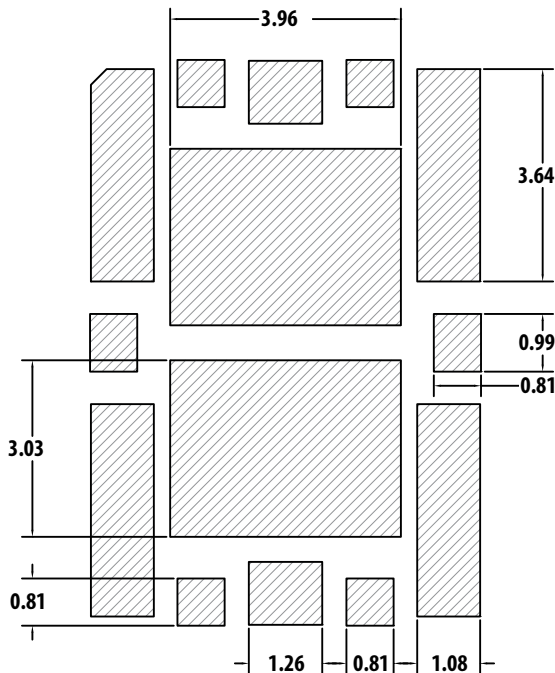
Stencil Outline
