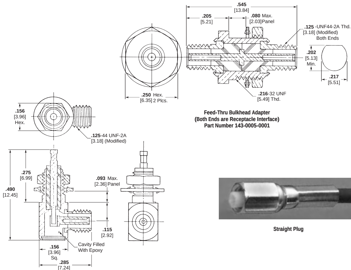
Right-Angle Receptacle 1 Part Number 141-0013-0001
