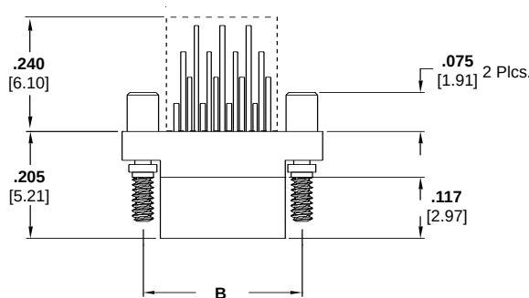
Receptacle Assembly Drawing Number 1589487
