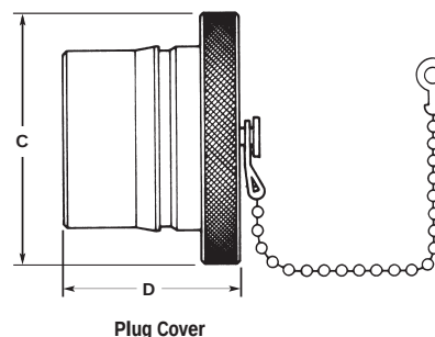
Plug Cover
