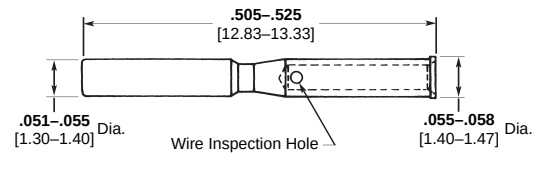
Part Number 082-0461-00Y9 (5-1532030-6) 22 AWG Socket
