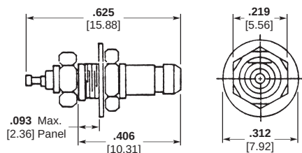
Receptacle, Rear Mount Part Number 145-0003-0001
