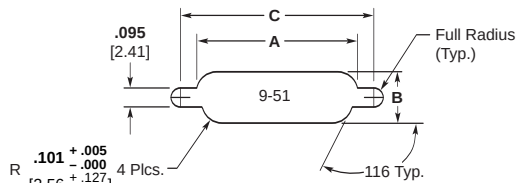
Figure 2 Rear Mounting
