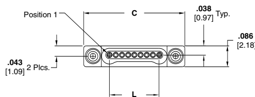
Plug with Flying Leads Drawing Number 1589455
