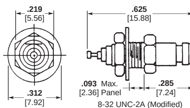
8-32 UNC-2A (Modified) Receptacle, Front Mount Part Number 145-0002-0001
