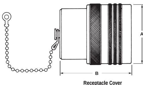
Receptacle Cover
