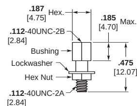
Part Number 6-1532137-4 Jackpost Assembly (S) S96-0002-0060 M83513/5-17
