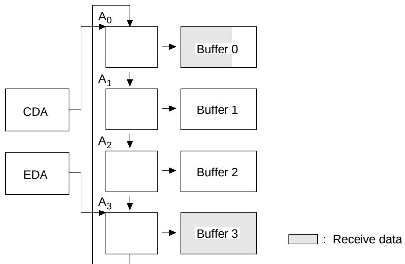
Figure 6.21 MSCI-to-Memory Chained-Block Multi-Frame Transfer (part of a buffer released during reception operation)
