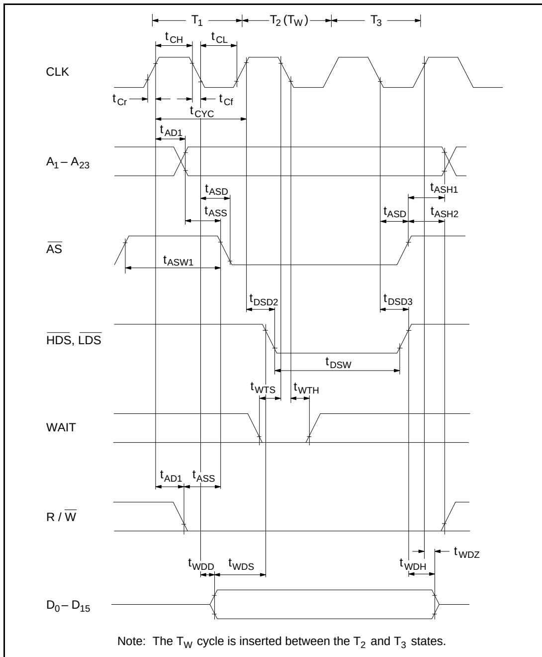
Figure 10.9 Master Mode Write Timing (CPU Mode 2, 3) (SCA \nleftrightarrow Memory)
