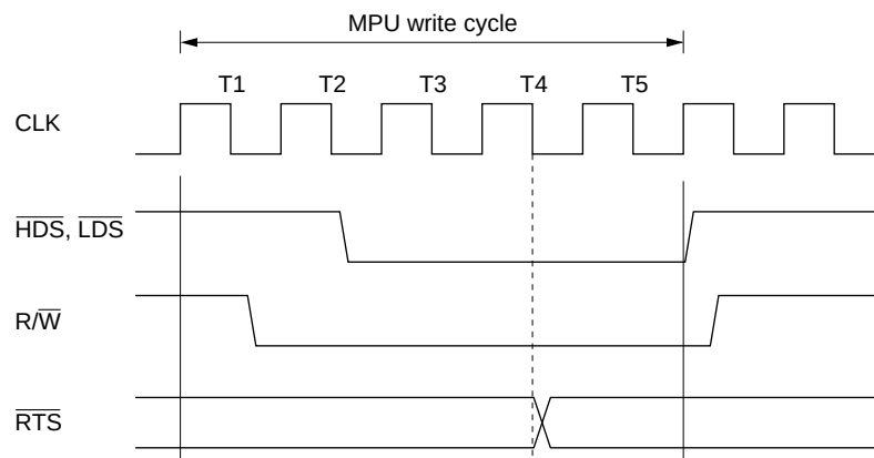
(e) CPU Mode 3, MPU Write Cycle
