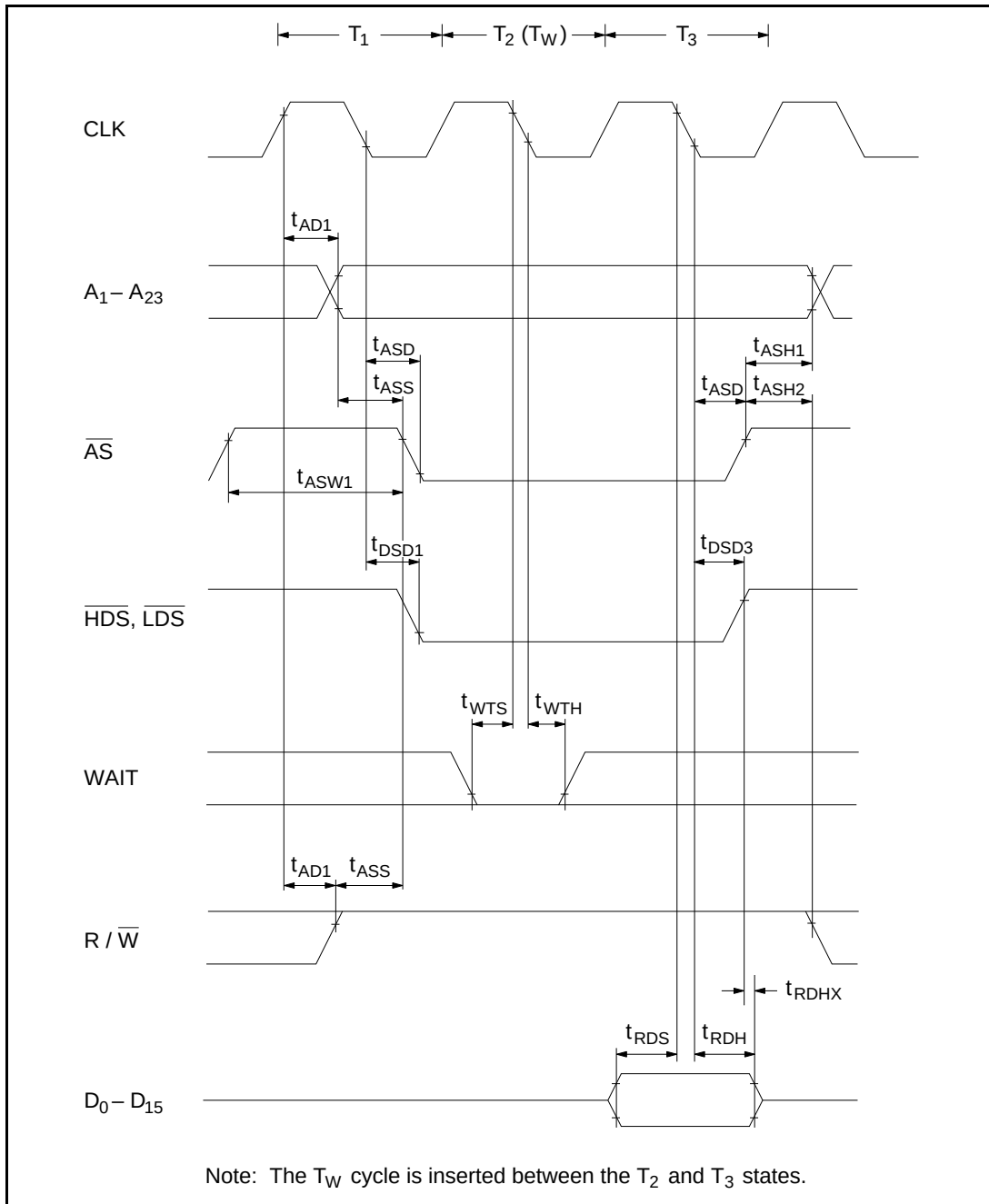
Figure 10.8 Master Mode Read Timing (CPU Mode 2, 3) (Memory \neq SCA)
