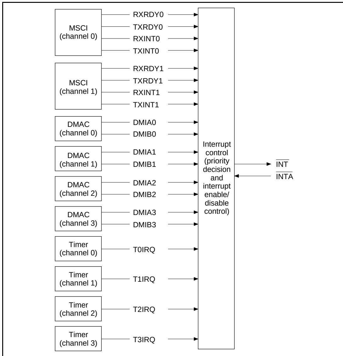
Figure 4.1 Interrupt Sources
