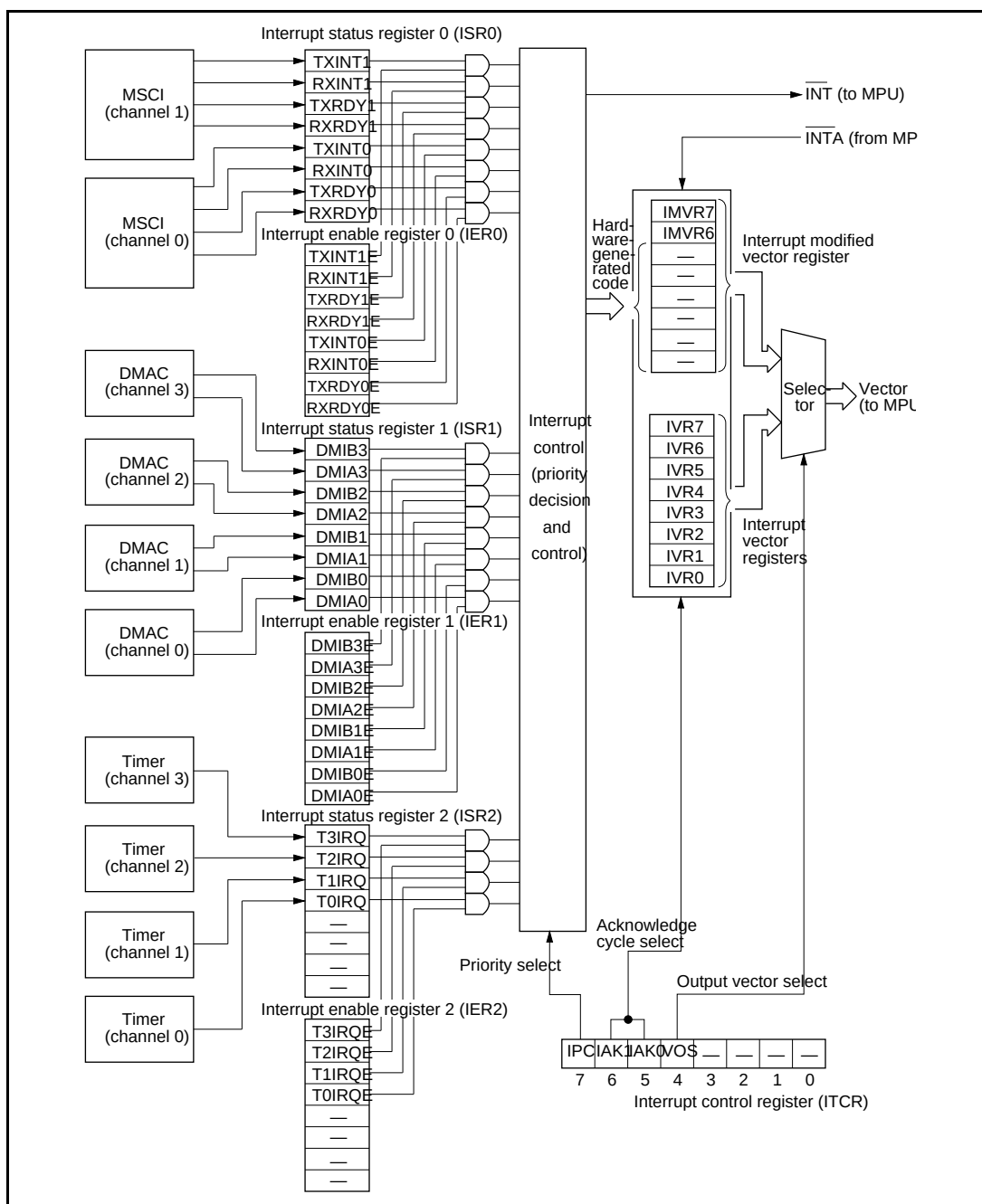
Figure 1.24 Interrupt Control
