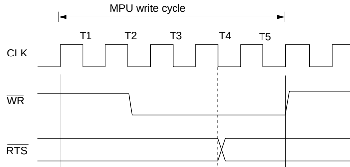
(c) CPU Mode 1, MPU Write Cycle
