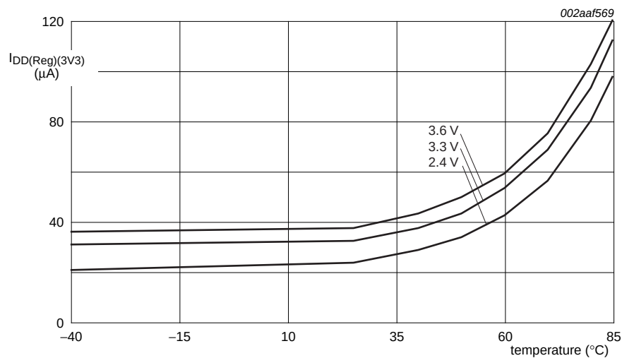
Fig 7. Power-down mode: Typical regulator supply current I_{DD(Reg)(3V3)} versus temperature
