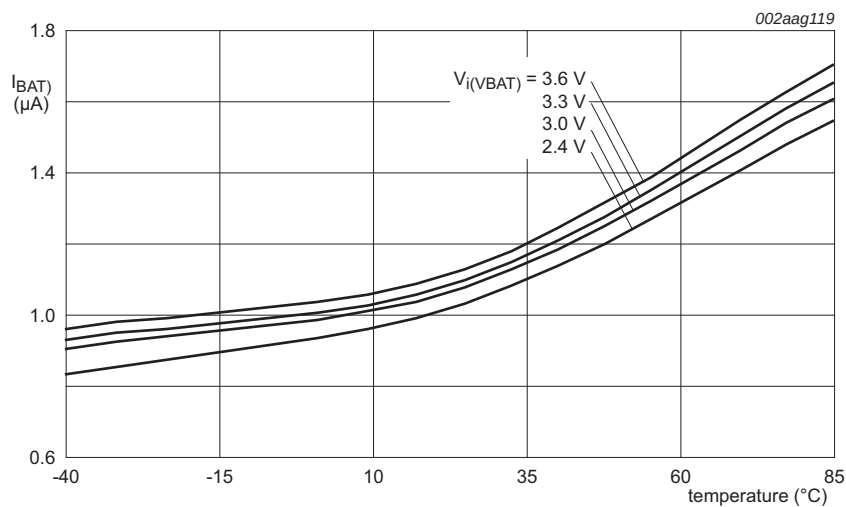
Fig 8. Deep power-down mode: Typical battery supply current I_{BAT} versus temperature
