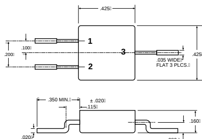
OM1324SMM
