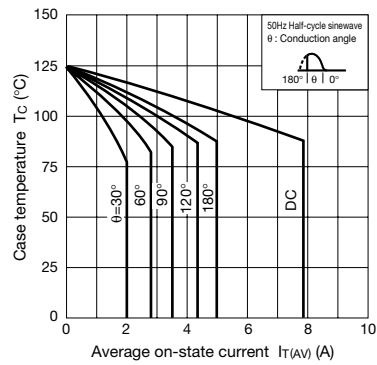
I_T(AV) - T_C Ratings
