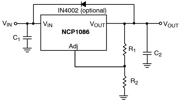
Figure 17. Protection Diode Scheme for Large Output Capacitors (Adjustable Output)
