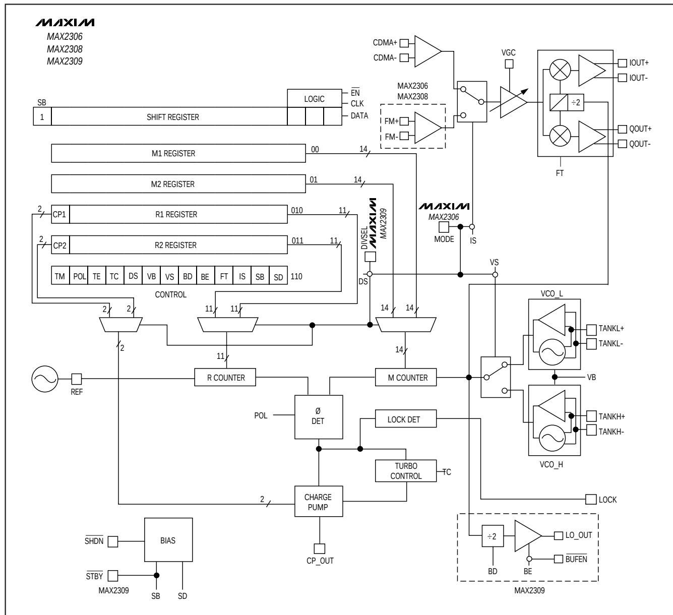
Functional Diagram
