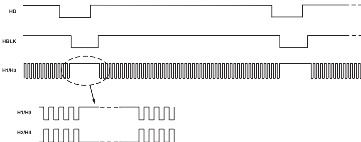
Figure 10. Horizontal Blanking (HBLK) Pulse Placement
