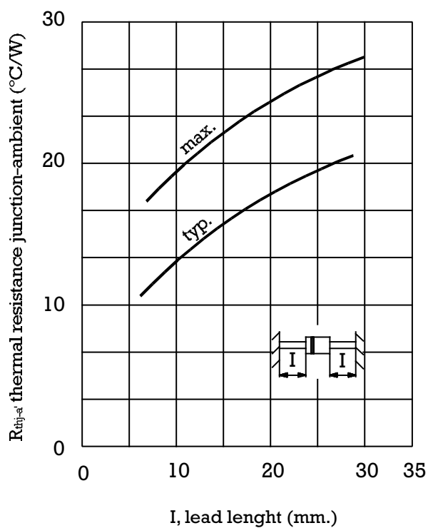
THERMAL RESISTANCE
