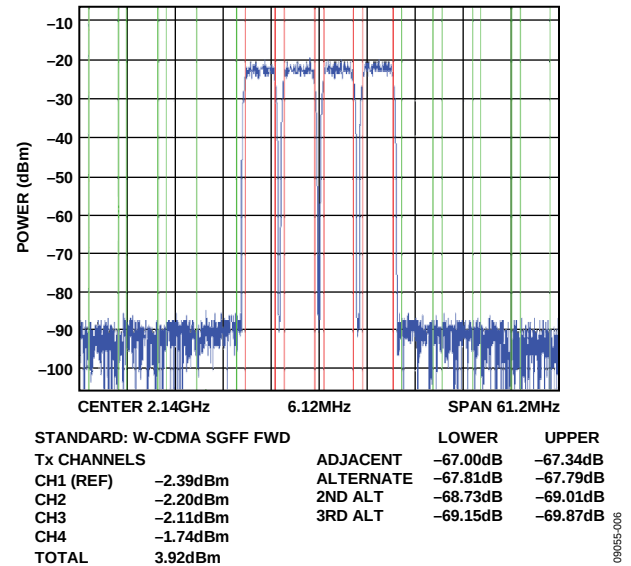
Figure 6. Four-Carrier W-CDMA Output
