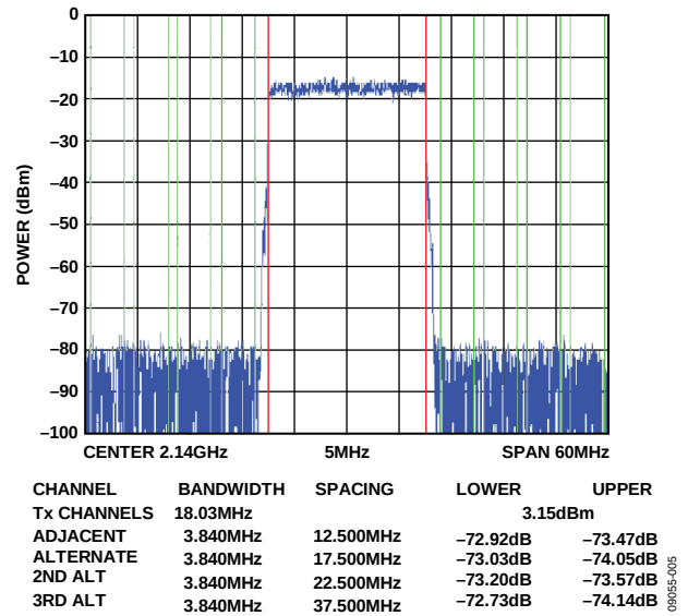
Figure 5. 20 MHz LTE Output
