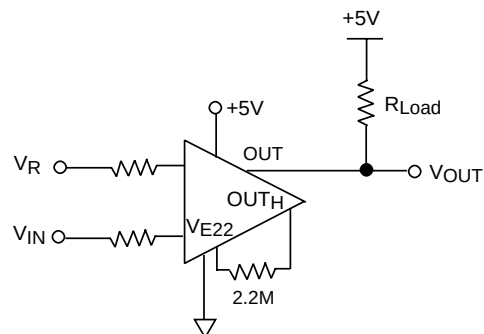
VOLTAGE COMPARATOR WITH OUTPUT FEEDBACK TO PROVIDE HYSTERESIS
