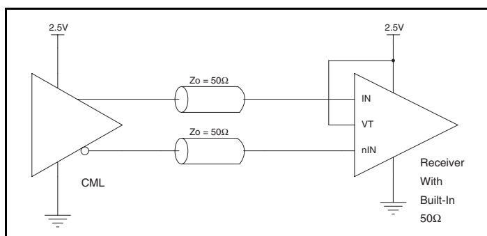
Figure 3C. HiPerClockS IN/nIN Input with Built-In 50 \Omega Driven by a CML Driver with Open Collector
