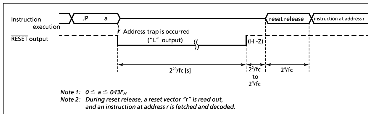
Figure 1-30. Address-Trap-Reset
