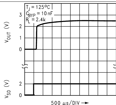
Figure 32. Turn-ON Waveform
