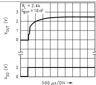
Figure 30. Turn-ON Waveform
