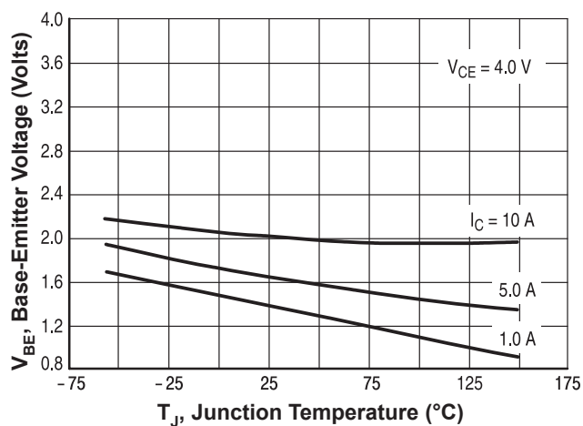
Base-Emitter Voltage
