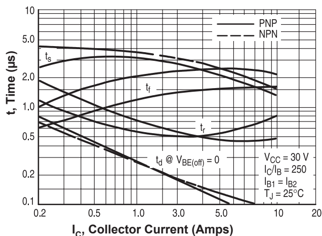
Switching Time
