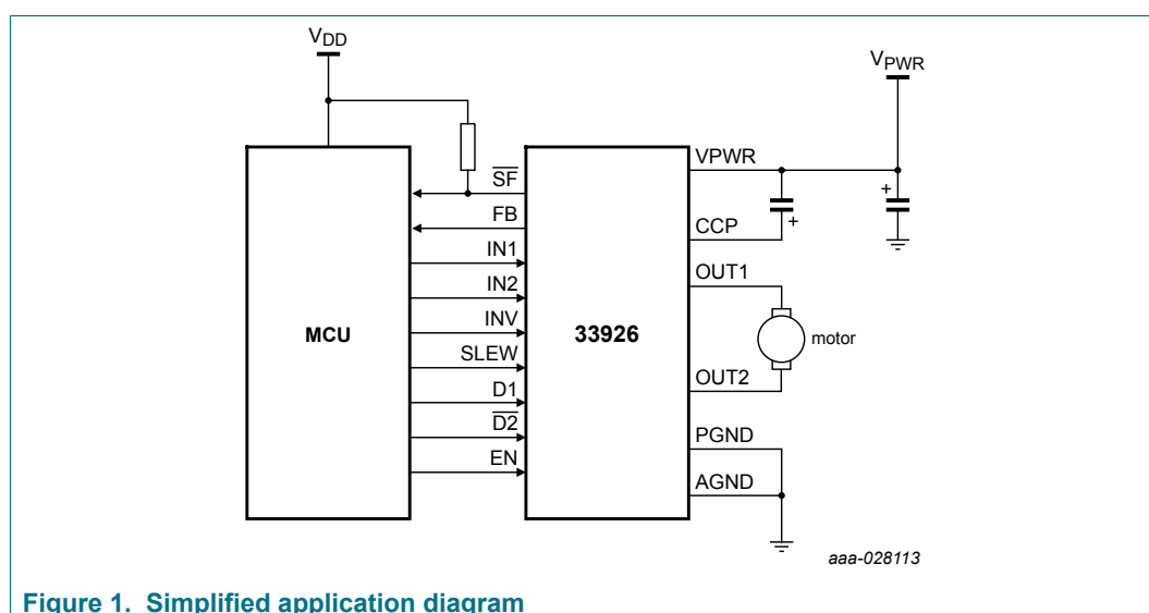
Figure 1. Simplified application diagram
