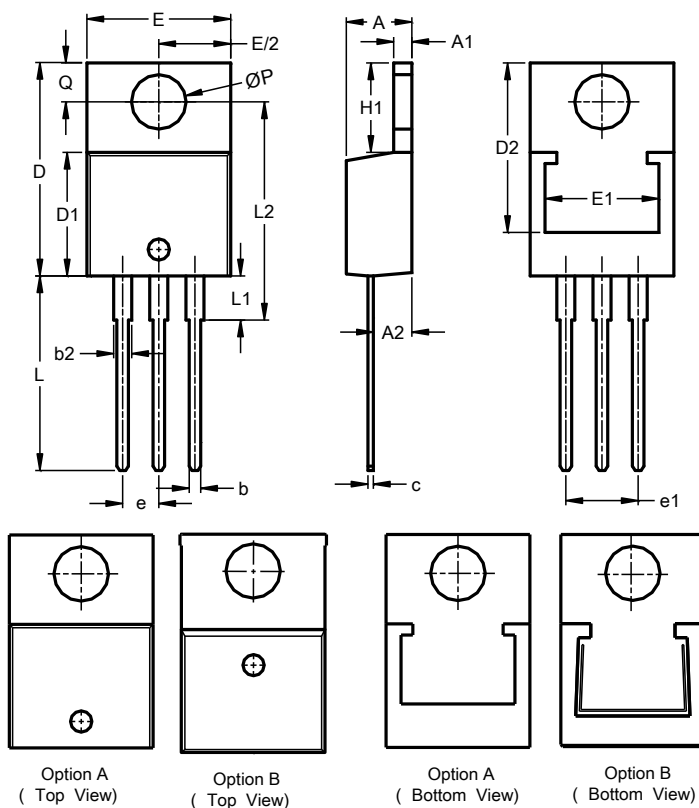
TO220AB (Generic)
