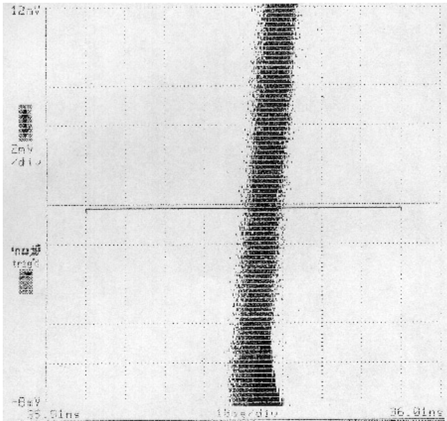
OP4012B Jitter Plot No Power Supply Noise
