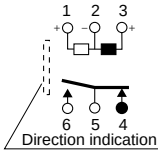
2-coil latching
