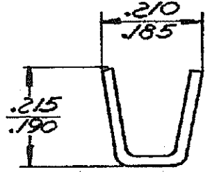
SECT. B-B
