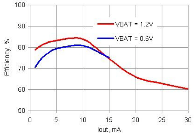
Figure 11-13. Efficiency vs I_{OUT} V_{BOOST} = 2.4\text{ V} , L_{BOOST} = 22\text{ }\mu\text{H}
