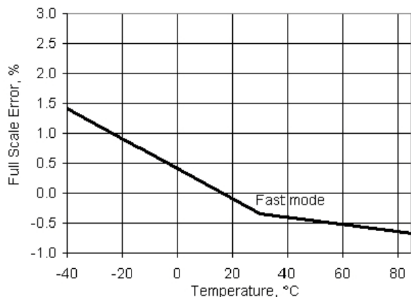
Figure 11-42. IDAC Full Scale Error vs Temperature, Range = 255 \mu A, Source Mode
