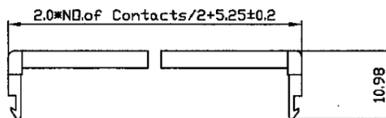
I.D.C SOCKET DUAL-ROW SR
