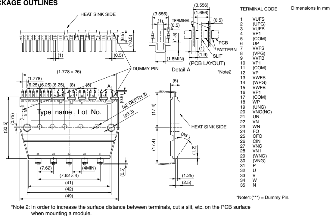
Fig. 1 PACKAGE OUTLINES
