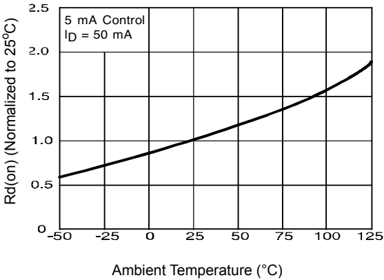
Figure 4. Typical On-Resistance
