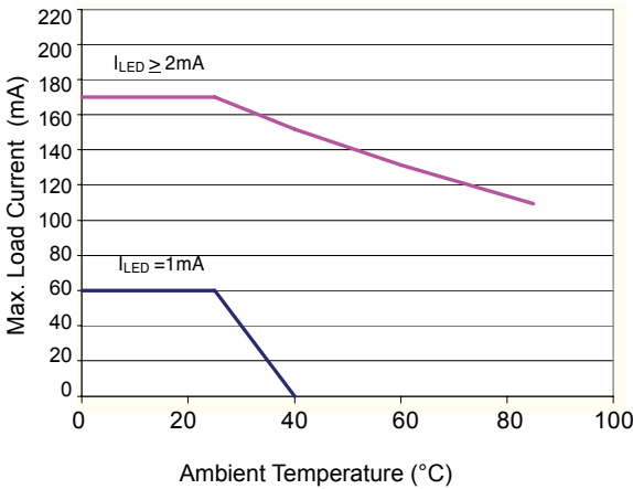
Figure 1. Current Derating Curves (PVA3324N)
