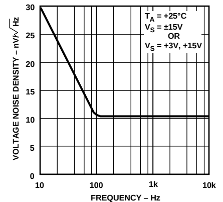
Figure 27. Voltage Noise Density vs. Frequency
