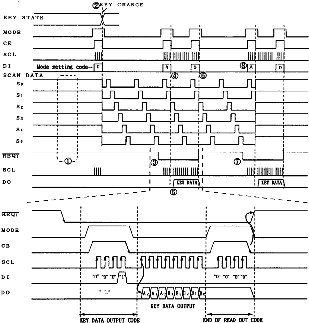
(3-3) Key Scan Timing Chart
