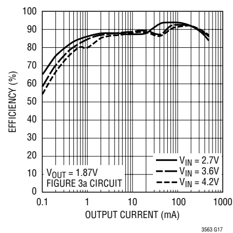
Figure 3c. Efficiency Curve
