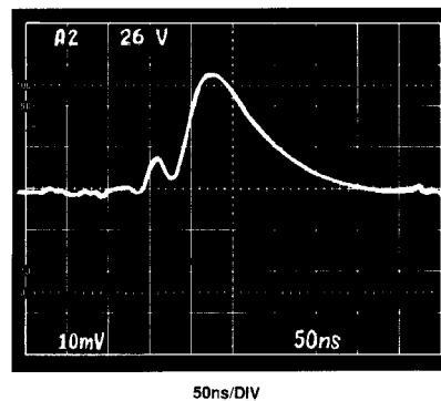
Figure 14. Digital Feedthrough
