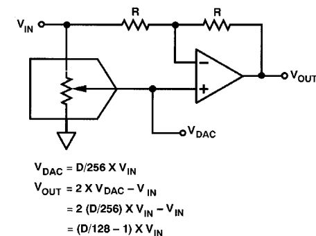
DAC8840 INPUT OUTPUT VOLTAGE RANGE
