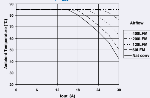
PT8120 Series, V_{out} = 1.5V
