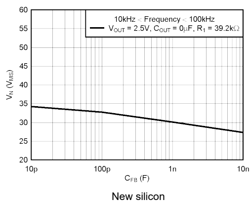
Figure 7-8. TPS73201 RMS Noise Voltage vs C FB
