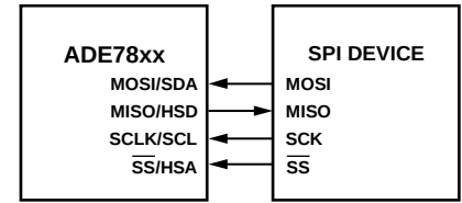
Figure 88. Connecting ADE78xx SPI with an SPI Device
