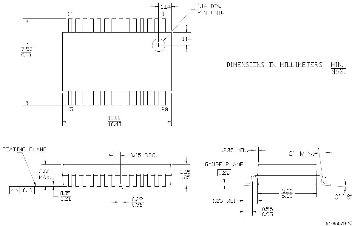
Figure 22-4. 28-Pin (5.3 mm) Shrunk Small Outline Package O28
