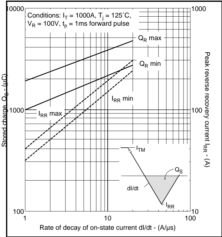
Fig.4 Stored charge
