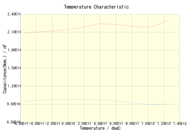
C2012X7R2E223K125AA(DC Bias = 0V) C2012X7R2E223K125AA(DC Bias = 125V)
