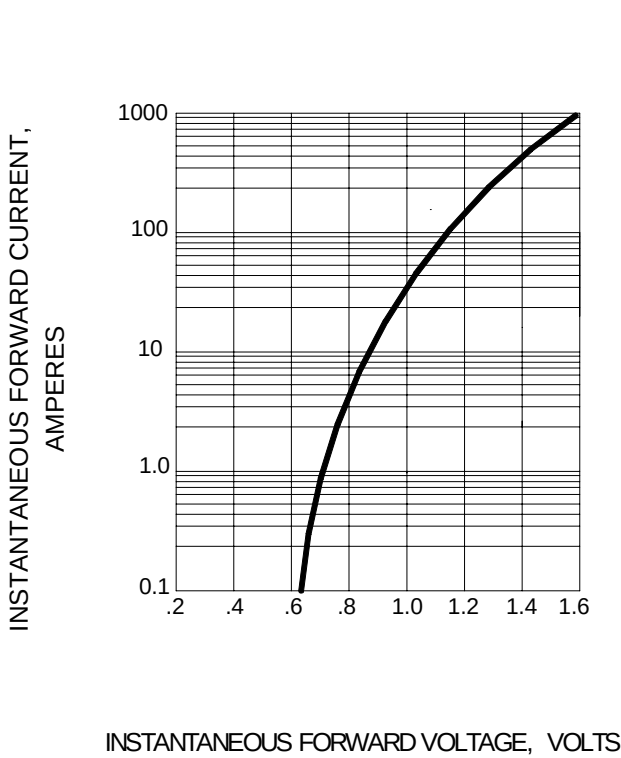
FIG.3 – TYPICAL FORWARD CHARACTERISTIC
