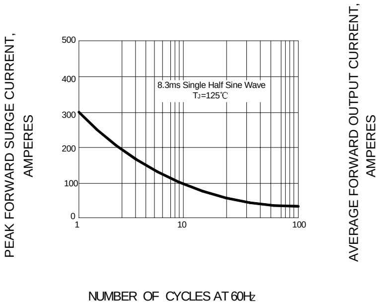
FIG.1 – PEAK FORWARD SURGE CURRENT
