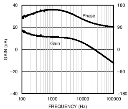
Figure 21. Modulator Gain and Phase - Buck Mode
