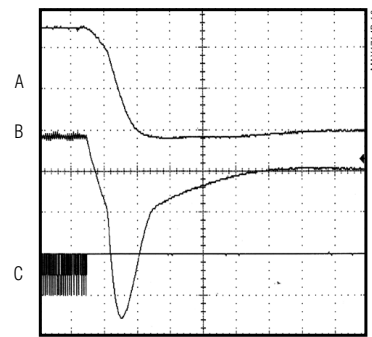
SHUTDOWN WAVEFORM (4A COMPONENTS, V_{OUT} = 2.5V , 300kHz)
