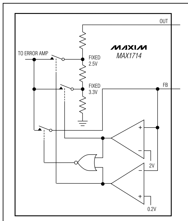
Figure 8. Feedback Mux
