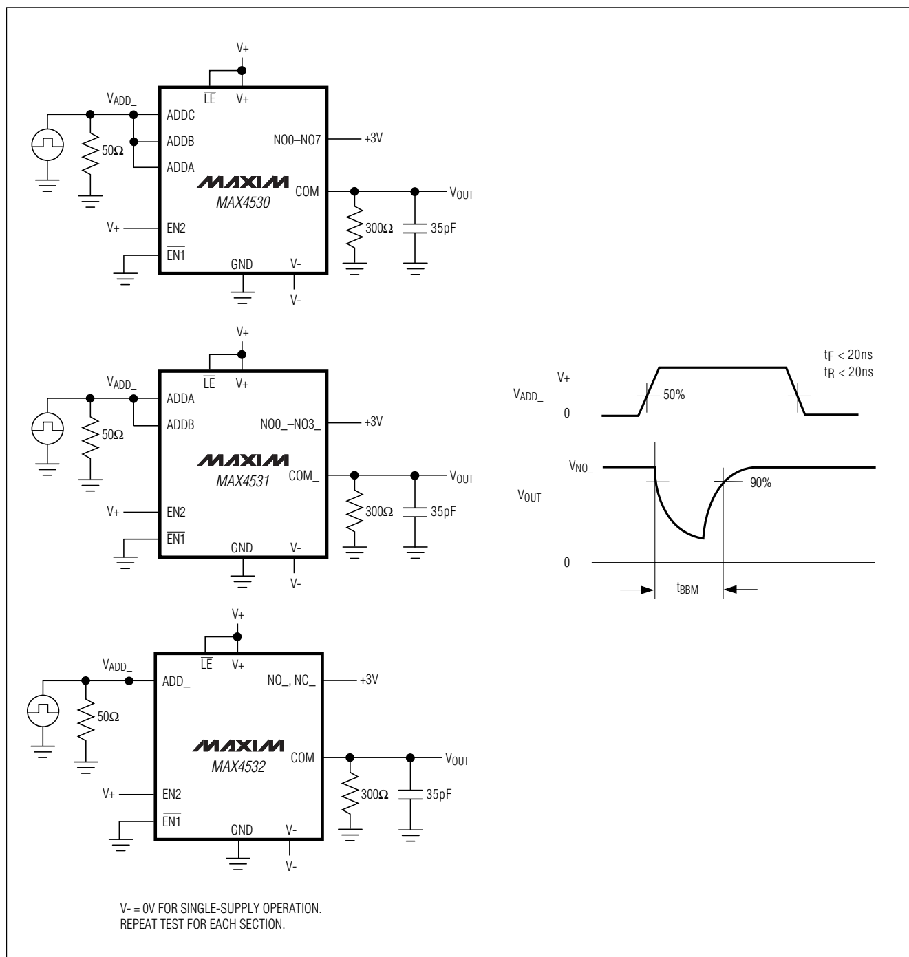
Figure 3. Break-Before-Make Interval
