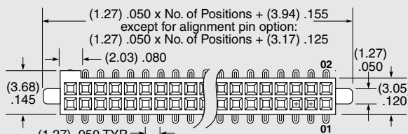
DOUBLE ROW
