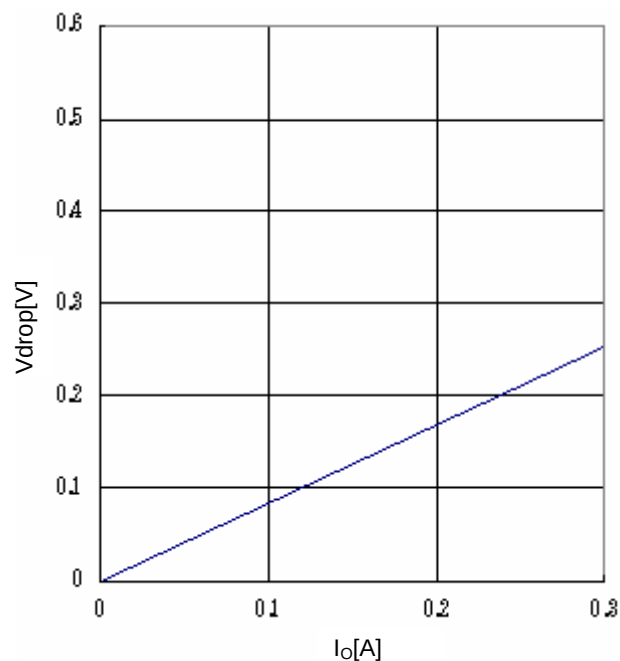
Fig.24 Minimum dropout Voltage 4 ( V_{CC}=8V , T_a=25^{\circ}C )
