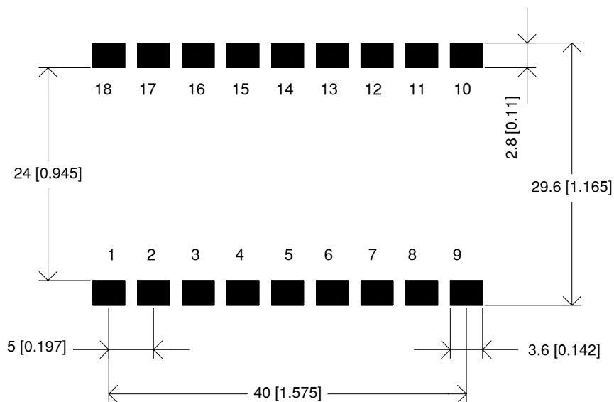
Recommended land pattern
